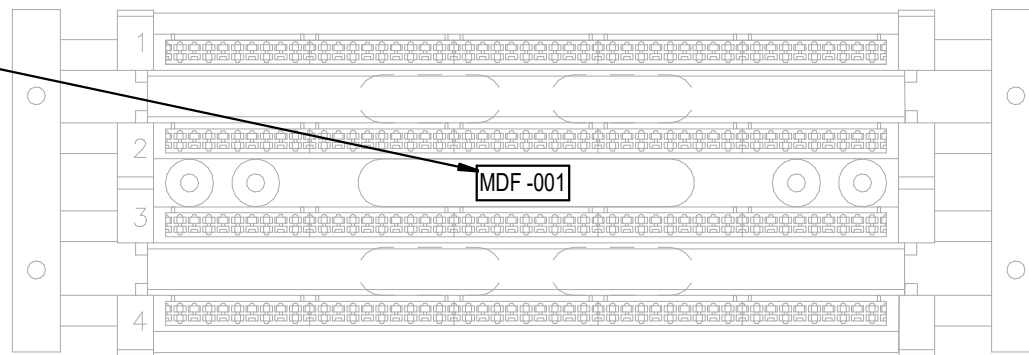
② Siemon S110A(X)2-100FT Labeling at IDF 6" = 1'-0"
