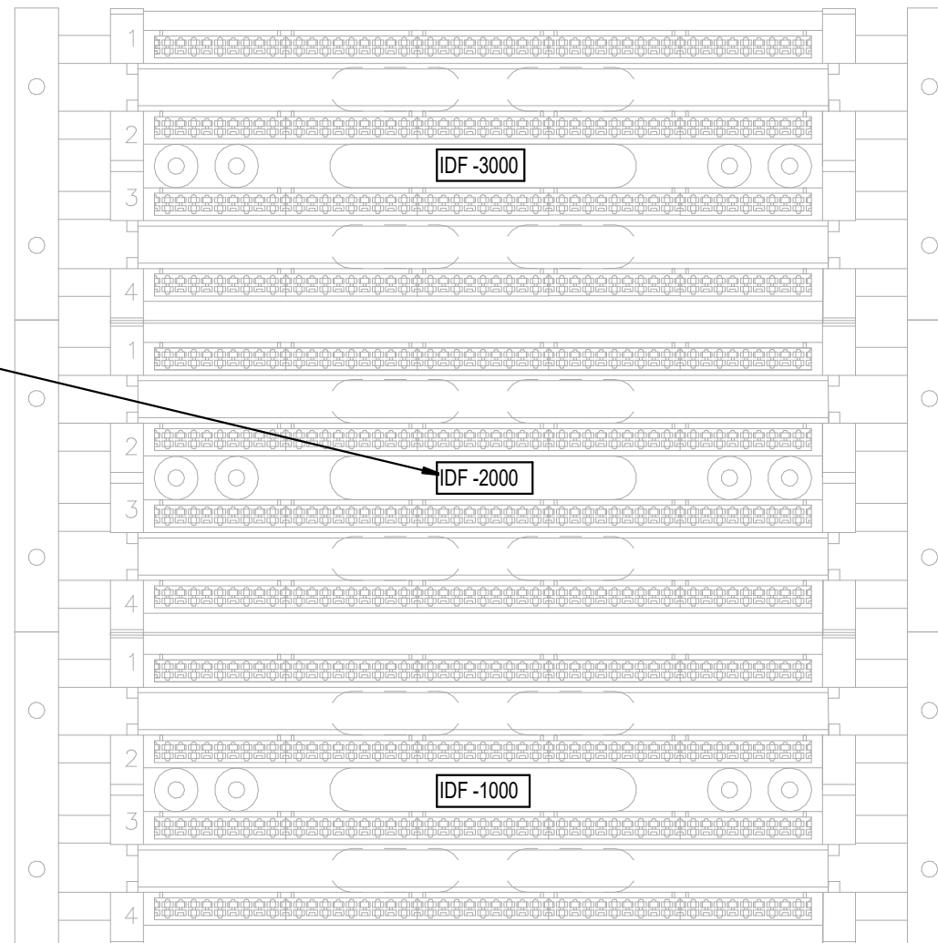
③ Siemon S110AA2-300FT Labeling at MDF 6" = 1'-0"
