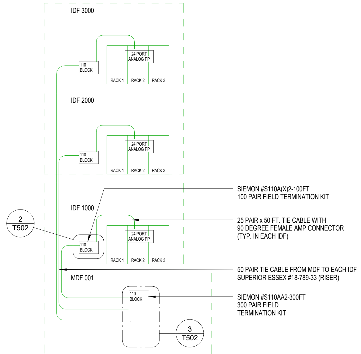
① Typical Copper Riser Diagram - Duke University 6" = 1'-0"
